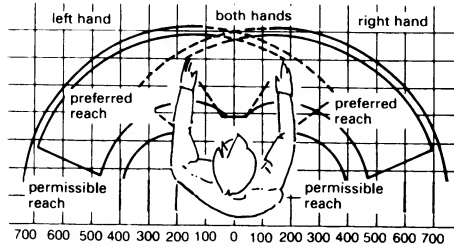
③ Preferred and permitted area of reach
